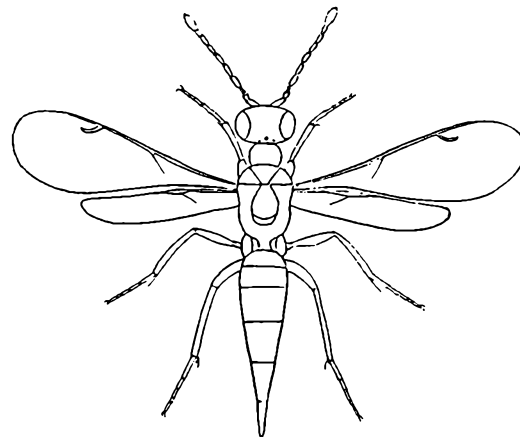
Photismus Thoms. (orig.)
