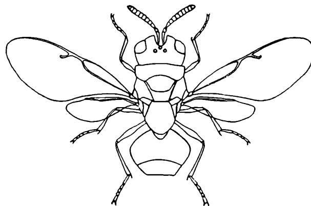
Perilampus Latr. (after Ashmead)
