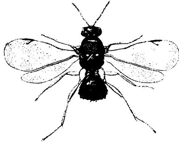
Euplectrus Westw. (after Thomsen)
