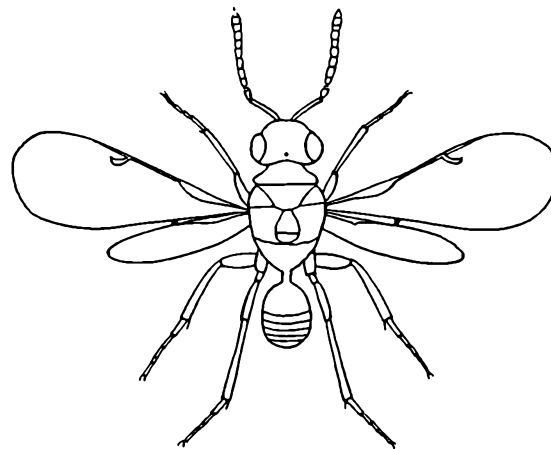
Polycystus Westw. (orig.)
