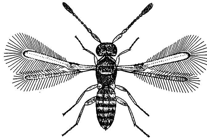
Cleruchus Enoch (after Bakkendorff)
