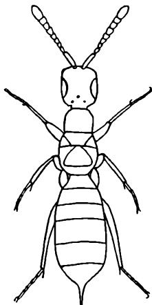
Theocolax West. (orig.)
