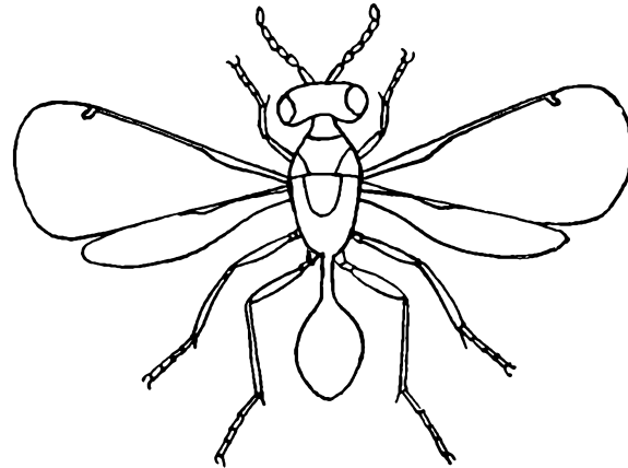
Derostenus Westw. (after Schmieck.)
