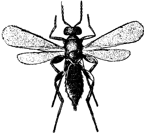
Elasmus Westw. (after Ahlberg)
