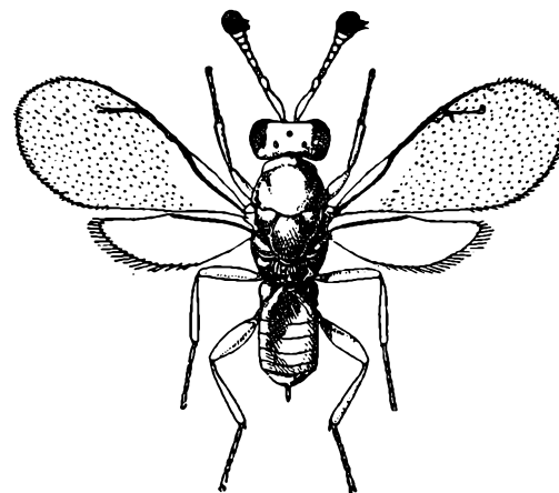
Eutelus Walk (after Mercet)
