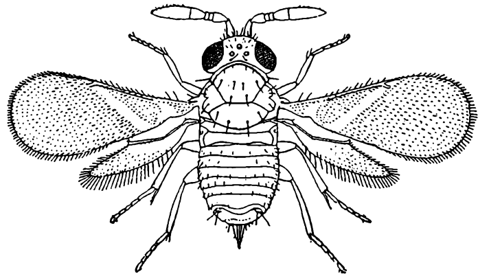
Aphelinus Dalm. (after Mercet)
