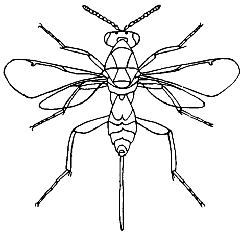
Callimome Spin. (after Huber)
