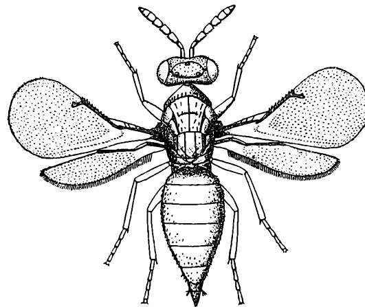
Tetrastichus Hal. (after Masi.)
