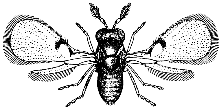
Ophioneurus Ratz. (after Bakkendorff)
