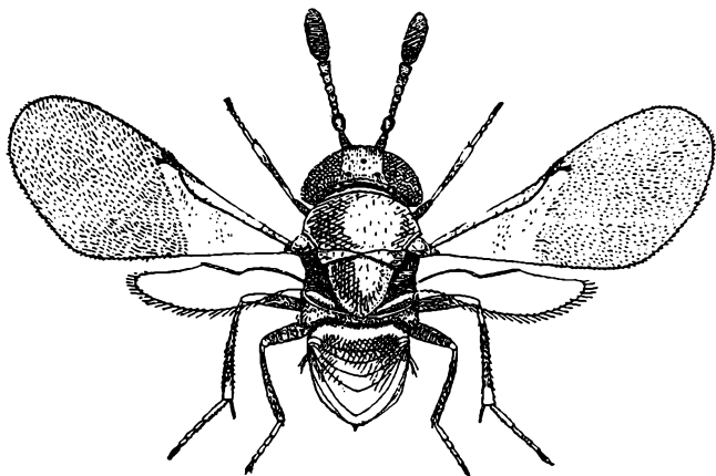
Aphidencyrthus Ashm. (after Mercet)
