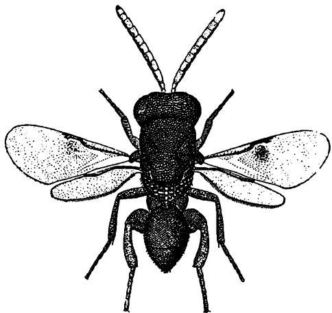
Chalcis Fabr. (after Masi.)
