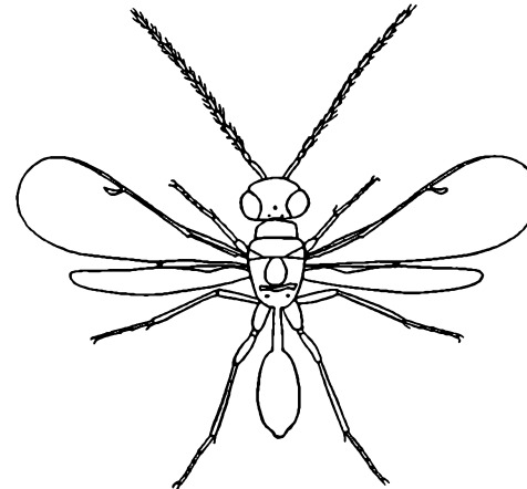
Dipara Walk. (orig.)
