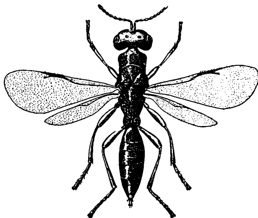
Harmolita Motsch. (after Gahan)
