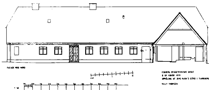
Facade mod nord.
