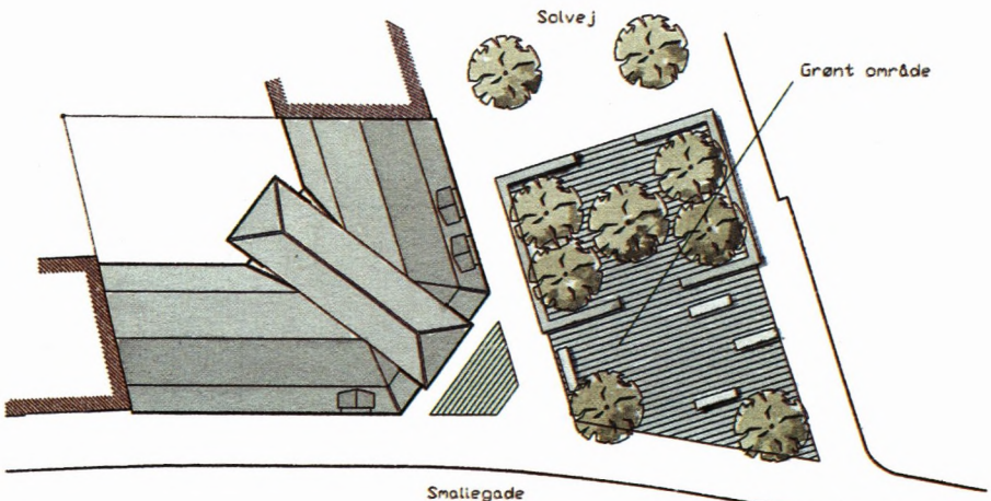
Situationsplan
