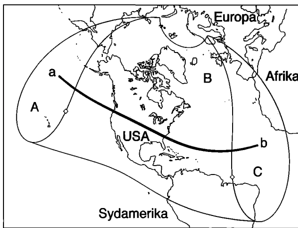
Total solformørkelse 21. august 2017
