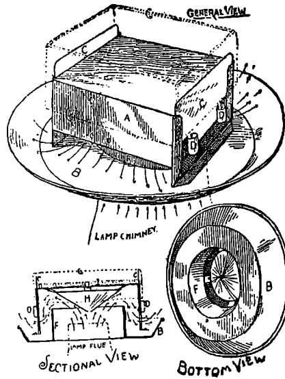
Fig. 56. Taylor's Tablesmelter.
