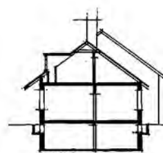
Snit f-f
