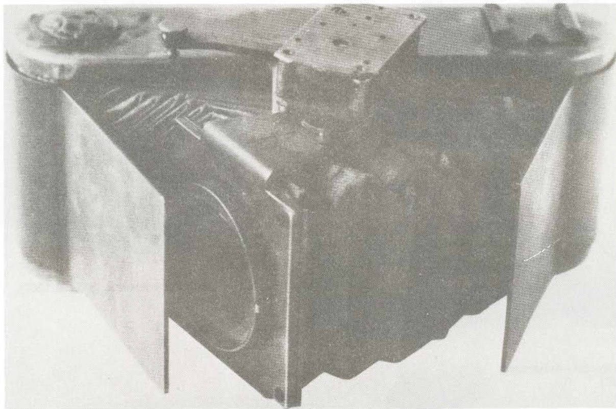
Leitz panoramakamera (prototype).
