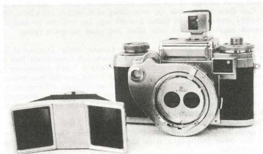
CONTAX IIA X STEREOTAR C. (1950-61).
