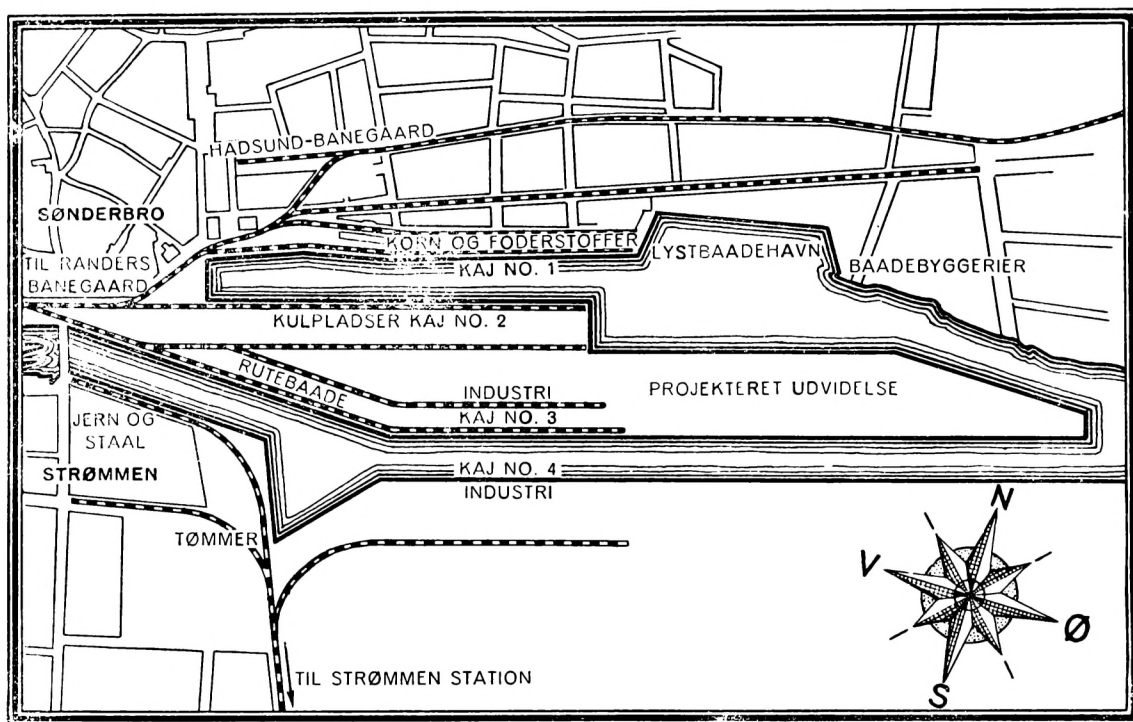
Plan over Randers ny Havn.
